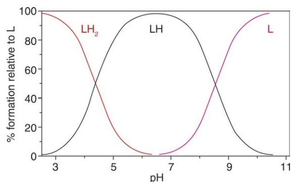
Fig. 3. Speciation diagrams of the PDPA, calculated for C_L = 2.0716 \text{ mmol dm}^{-3} , at 25^\circ\text{C} and I = 0.1 \text{ mol dm}^{-3} (KCl).
