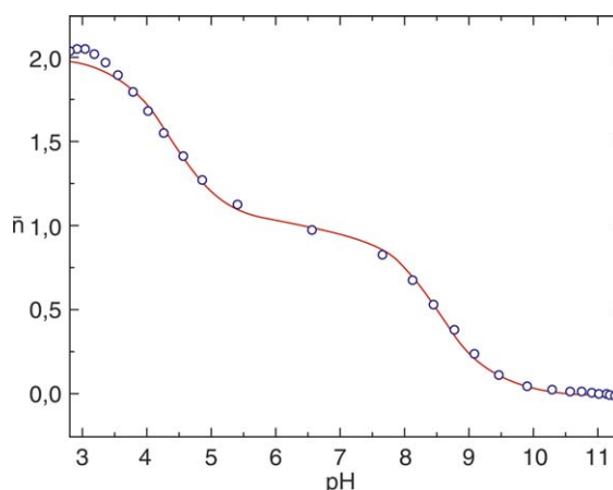
Fig. 2. Protonation curves for ligand; solid line represents calculated function from potentiometric data, circles represent experimental protonation curve. Both curves were obtained for C_L = 2.0716 \text{ mmol dm}^{-3} at 25 °C and I = 0.1 \text{ mol dm}^{-3} (KCl).
