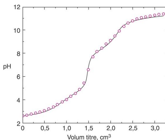
Fig. 1. Experimental titration curve (circle) and simulation titration curve (solid line) for C_L = 2.0716 \text{ mmol dm}^{-3} at 25 °C and I = 0.1 \text{ mol dm}^{-3} (KCl).
