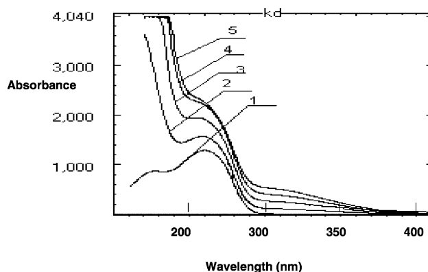
Fig. 2. Absorption spectra: 1 , KD ( 4 \times 10^{-5} mol l -1 ); 2 , KD ( 4 \times 10^{-5} mol l -1 ) + Fe(III) ( 8 \times 10^{-5} mol l -1 ); 3 , KD ( 4 \cdot 10^{-5} mol l -1 ) + Fe(III) ( 1.6 \times 10^{-4} mol l -1 ); 4 , KD ( 4 \times 10^{-5} mol l -1 ) + Fe(III) ( 3.2 \times 10^{-4} mol l -1 ); 5 , KD ( 4 \cdot 10^{-5} mol l -1 ) + Fe(III) ( 6.4 \times 10^{-4} mol l -1 ) at pH = 1.6.
