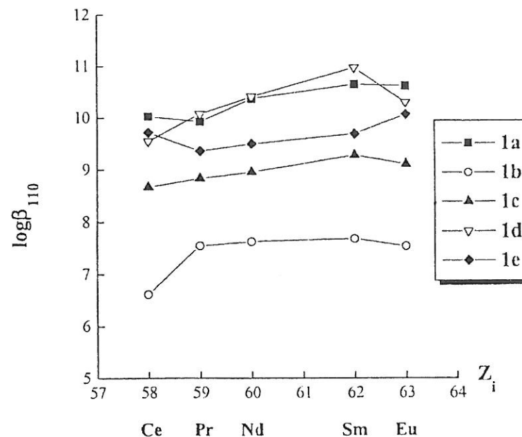
FIGURE 5 Variation of \log \beta_{110} of complexes versus the atomic number of \text{Ce}^{3+} , \text{Pr}^{3+} , \text{Nd}^{3+} , \text{Sm}^{3+} , and \text{Eu}^{3+} .
