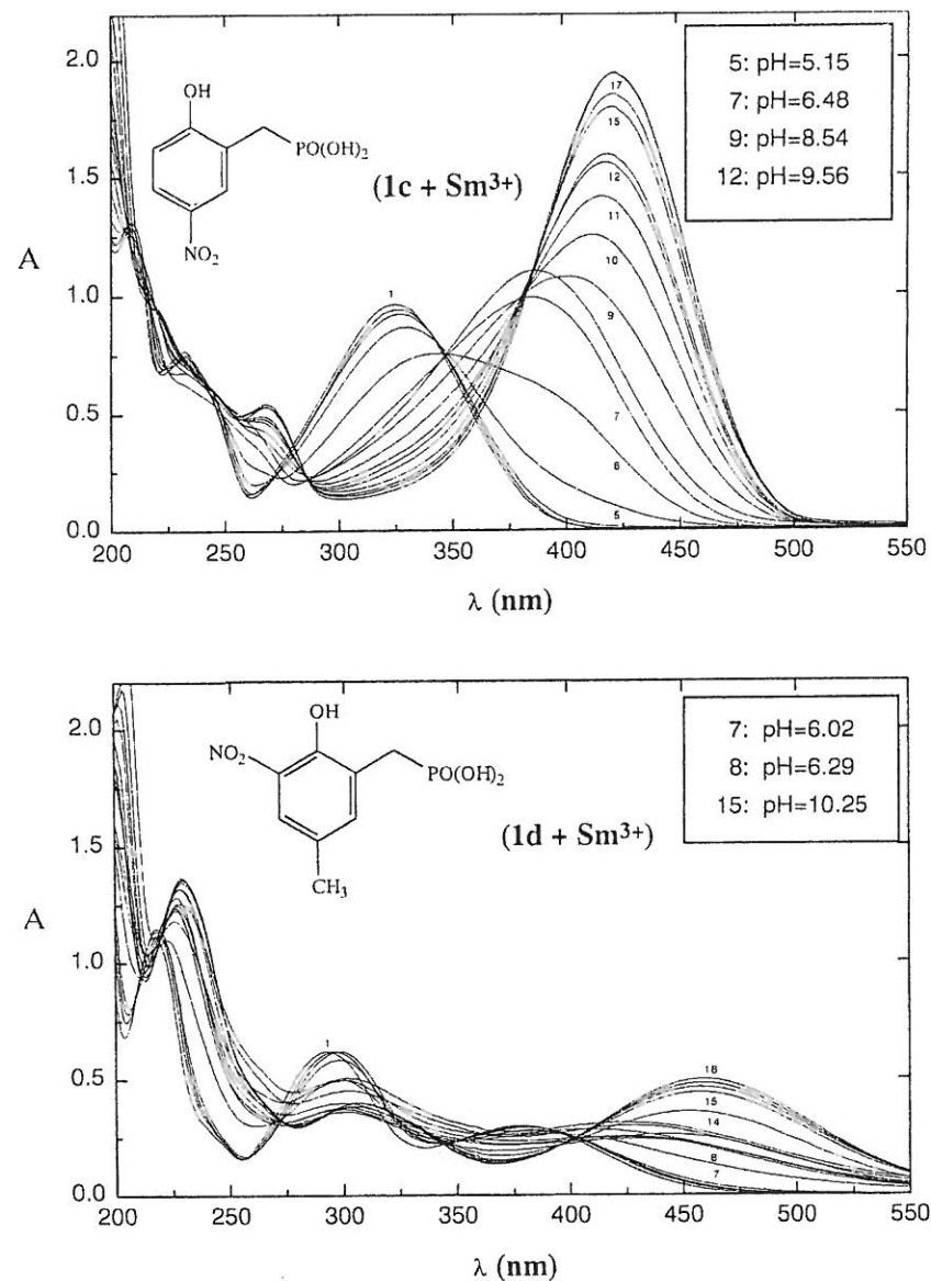
FIGURE 2 Experimental absorption spectra of 1c and 1d complexes with \text{Sm}^{3+} .
