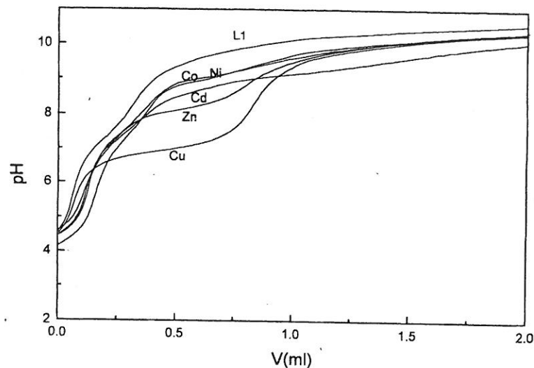
FIGURE 2 Neutralisation curves of L1 ( 10^{-4} mol.L ^{-1} ) by NaOH ( 10^{-2} mol.L ^{-1} ) in the absence and in presence of the metal cations ( 10^{-4} mol.L ^{-1} ) at 25 °C and with I = 0.1 mol.L ^{-1}
