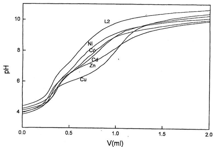
FIGURE 3 Neutralisation curves of L2 ( 10^{-4} mol.L ^{-1} ) by NaOH ( 10^{-2} mol.L ^{-1} ) in the absence and in presence of the metal cations ( 10^{-4} mol.L ^{-1} ) at 25°C and with I = 0.1 mol.L ^{-1}
