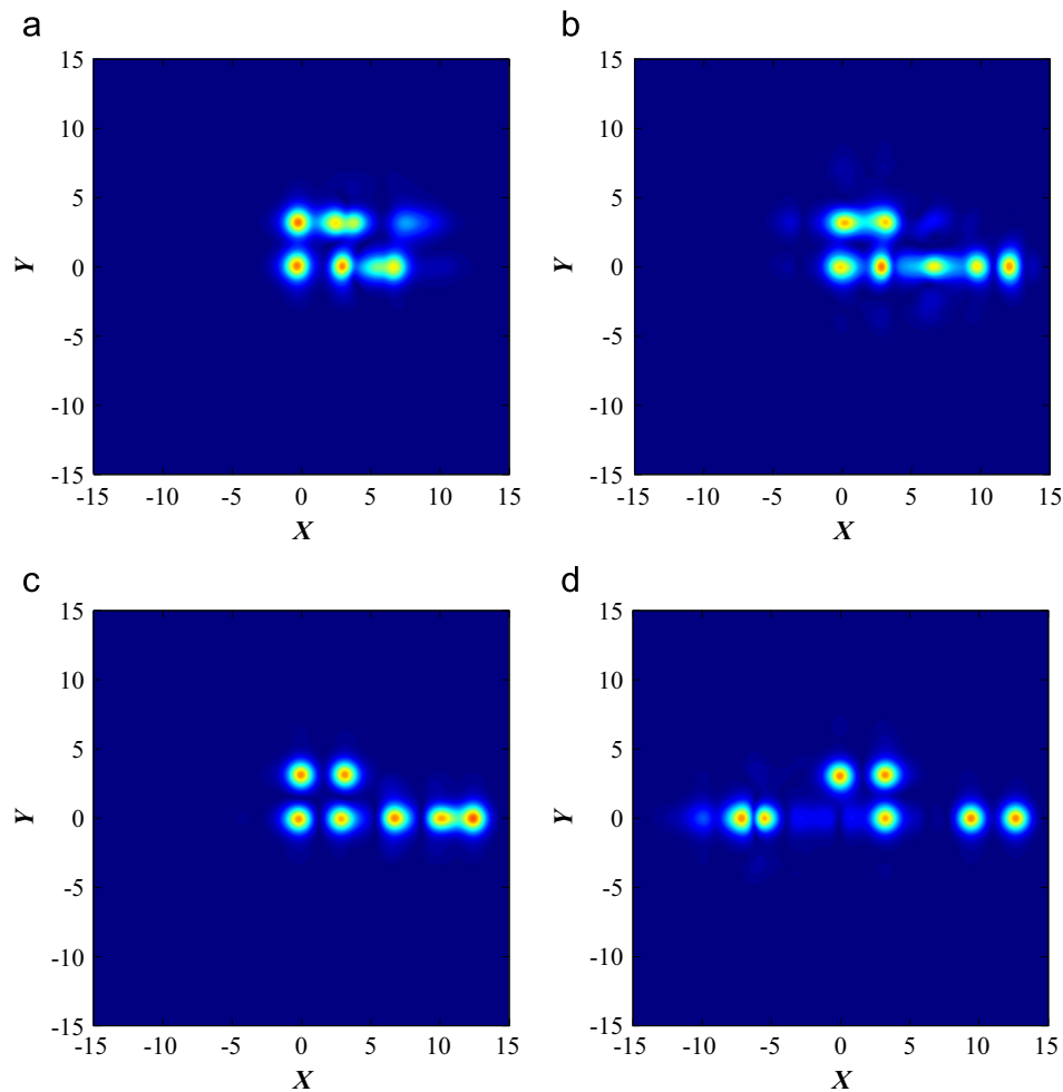
Fig. 17. The evolution of the unstable offsite-centered vortex kicked in the horizontal direction ( \theta = 0 ) with k_0 = 1.5 . The color code is the same as in Fig. 1(a). (a) Z=2.6593 , (b) Z=12.008 , (c) Z=239.91 , and (d) Z=299.825 .
