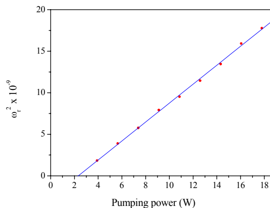
Fig. 3. Evolution of the square of the eigenfrequency versus the pumping power.
