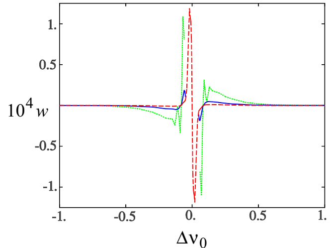
Fig. 10. Soliton inverse velocity w = \Delta t / \Delta z against detuning \Delta\nu_0 = \Delta\omega_0 / 2\pi for a few values of the injected cw amplitude, namely A = 0.004 (green dotted line), 0.002 (red dashed line), and 0.001 (blue solid line). (For interpretation of the references to colour in this figure legend, the reader is referred to the web version of this article.)
