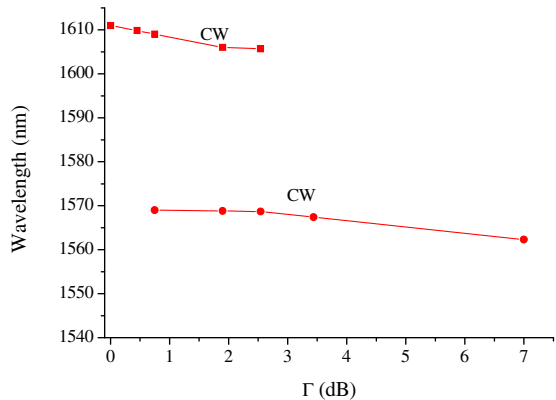
Fig. 8. Evolution of the oscillating wavelengths as a function of additional losses \Gamma for the ring cavity.
