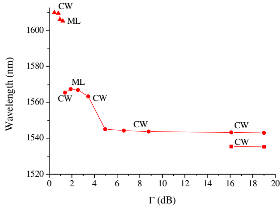
Fig. 5. Evolution of the oscillating wavelengths as a function of additional losses \Gamma for the F8L.
