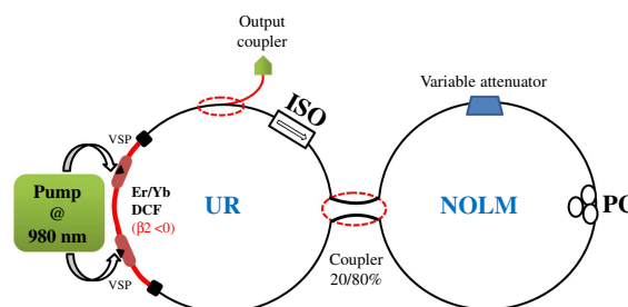
Fig. 1. F8L schematic.
