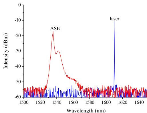
Fig. 2. Optical spectra of the laser and ASE.
