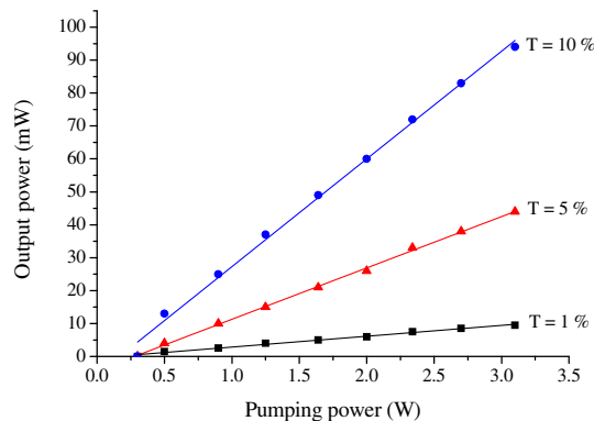
Fig. 3. Output power at 1610 nm versus the pumping power, for different output coupling ratios T , for the F8L.
