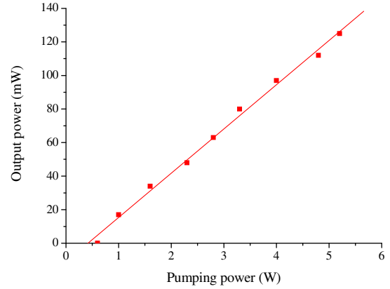
Fig. 7. Evolution of the output power at 1611 nm versus the pumping power for the ring cavity.
