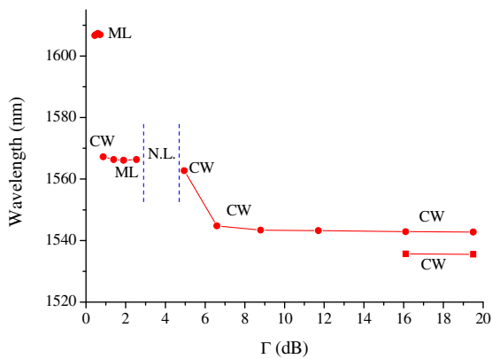
Fig. 6. Evolution of the oscillating wavelengths as a function of additional losses \Gamma for the F8L, but with a different orientation of the polarization controller. N.L. stands for noise-like emission.
