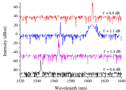
Fig. 4. Evolution of the optical spectrum as a function of the additional losses \Gamma for the F8L.
