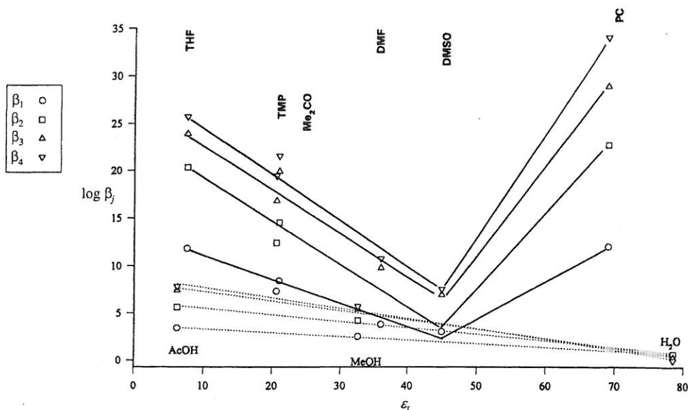
Figure 1. A plot of \log \beta_j of the copper(II) chloro complexes versus the dielectric constant \epsilon_r of the nine solvents studied. Dotted lines, protic solvents; solid lines, aprotic solvents.
