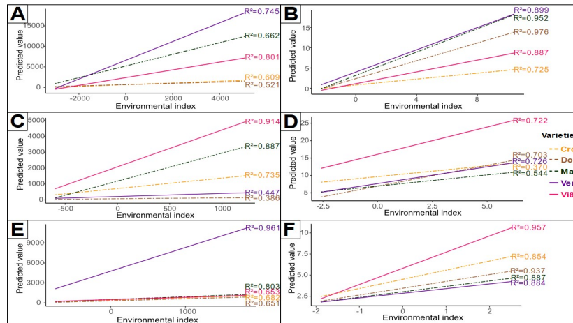
Fig 5. Environmental sensitivity of five varieties for six compounds over 20 environments. (A) PP2 myristicin, (B) 6MM 6-methoxymellein, (C) S6 D-germacrene, (D) FaDOAc falcarindiol acetate, (E) T2 \beta -pinene and (F) acar \alpha -carotene. X-axis represents environmental index for compounds synthesis all varieties combined, and Y-axis level of predicted synthesis for each variety. Slope is traced according to regression coefficient bi (S3 Table).
