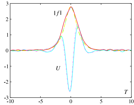
Fig. 2. Initial (at Z = 100 ) and final (at Z = 40,000 ) profiles of a CP FCP soliton. The initial data is composed of one mKdV breather (53) for each polarization component, with a \pi/2 dephasing between them. The parameter used is p_1 = 1 + 1.5i , which correspond to a ratio of the angular frequency divided by the pulse length of 1.5. Blue (dotted): initial |f| , light blue (thick solid, gray): initial U , red (solid black): final |f| , pink (dash-dotted): final U . The green (thin dashed) and yellow (thick dashed, gray) lines are fits using the analytical approximate profile (52).
