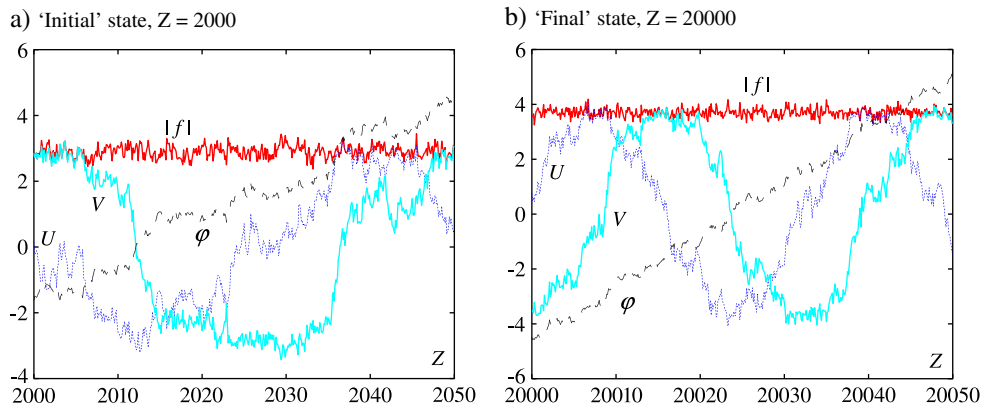
Fig. 6. One period of rotation of the slowly rotating LP half-cycle pulse resulting from the instability of the CP FCP with both angular frequency and pulse length 1, at the beginning of its evolution (a), and after long propagation (b). Red (thin solid): norm of the electric field |f| , blue (dotted): x-polarized component U , light blue (thick solid gray): y-polarized component V , black (dashed): phase \arctan(V/U) .
