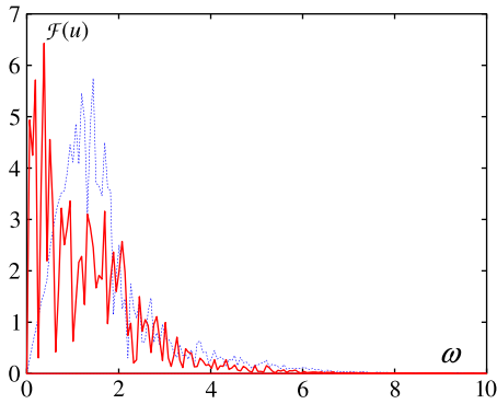
Fig. 3. Optical spectrum of an unstable CP FCP just before (at Z = 400 , blue dotted line) and just after its decay (at Z = 500 , red solid line) into slowly rotating LP half-cycle pulse. Initial data is based on Eq. (53) with p_1 = 1 + i , which correspond to an angular frequency equal to the pulse length.
