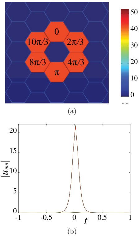
FIG. 9. (Color online) The same as in Fig. 6 but for a stable hexagonal vortex with topological charge S = 2 , generated by the modified input with \mu = 223 .
