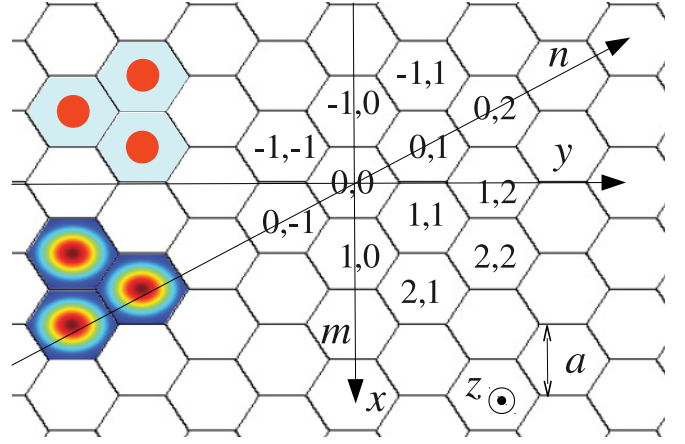
FIG. 1. (Color online) The setup and notation: We consider the hexagonal array of cylindrical waveguides, as shown in the upper left corner. The transverse distribution of the light intensity of the propagating waves in the guiding cores is displayed symbolically in the bottom left corner. Each core is assumed to be a single-mode waveguide, represented by wave function u_{m,n} , with discrete coordinates (m,n) defined as shown in the figure. The map of integers m,n into the Cartesian coordinates in the transverse plane, (x,y) , is performed as per Eq. (5), a being the width of the hexagonal cell.
