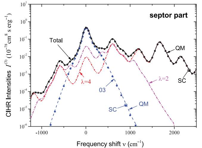
FIG. 4. (Color online) The CIHR binary polarized sector spectrum I_{\perp}^{(3)} (in \text{cm}^8 \text{ s erg}^{-1} ) of the H 2 -Ne pair at T = 295 \text{ K} , versus frequency shift ( \nu , in \text{cm}^{-1} ) with regard to the central frequency 4\pi c/\lambda_L (where \lambda_L = 1064 \text{ nm} is the exciting laser wavelength). The semiclassical spectra are denoted by dots and labeled by SC, whereas the quantum spectrum is plotted with lines (dash or solid) and labeled by QM; a discussion of the result uncertainties is within the text (Secs. IV A and IV B).
