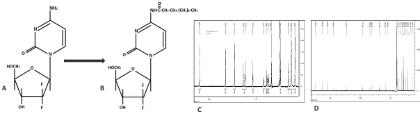
A. Gemcitabine. B. 4-(N)-lauryl-gemcitabine. C-D. 1 H NMR and 13 C NMR Spectrum of 4-(N)-lauryl-gemcitabine
