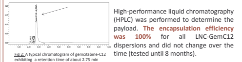
Fig. 2. A typical chromatogram of gemcitabine-C12 exhibiting a retention time of about 2.75 min
