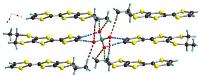
Figure 3. Solid-state structure of [( R )-1] 2 ClO 4 , with an emphasis on the C–H⋯O short contacts: blue dotted lines for CH vinylyl (2.43–2.51 Å), green dotted lines for CH 2 (2.46–2.63 Å), brown dotted lines for Me (2.62 Å) and red dotted line for CH Me (2.99 Å).
