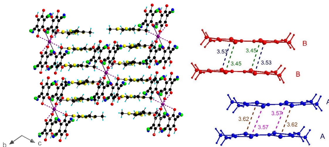
Figure 2. View of the crystal structure of compound 1 along a (left). Short S\cdots S contacts (Å) between AA and BB dimer molecules shorter than sum of van der Waal radii (3.65): S1A-S4A 3.57; S2A-S3A 3.62; S5B-S8B 3.45; S6B-S7B 3.53 (right).
