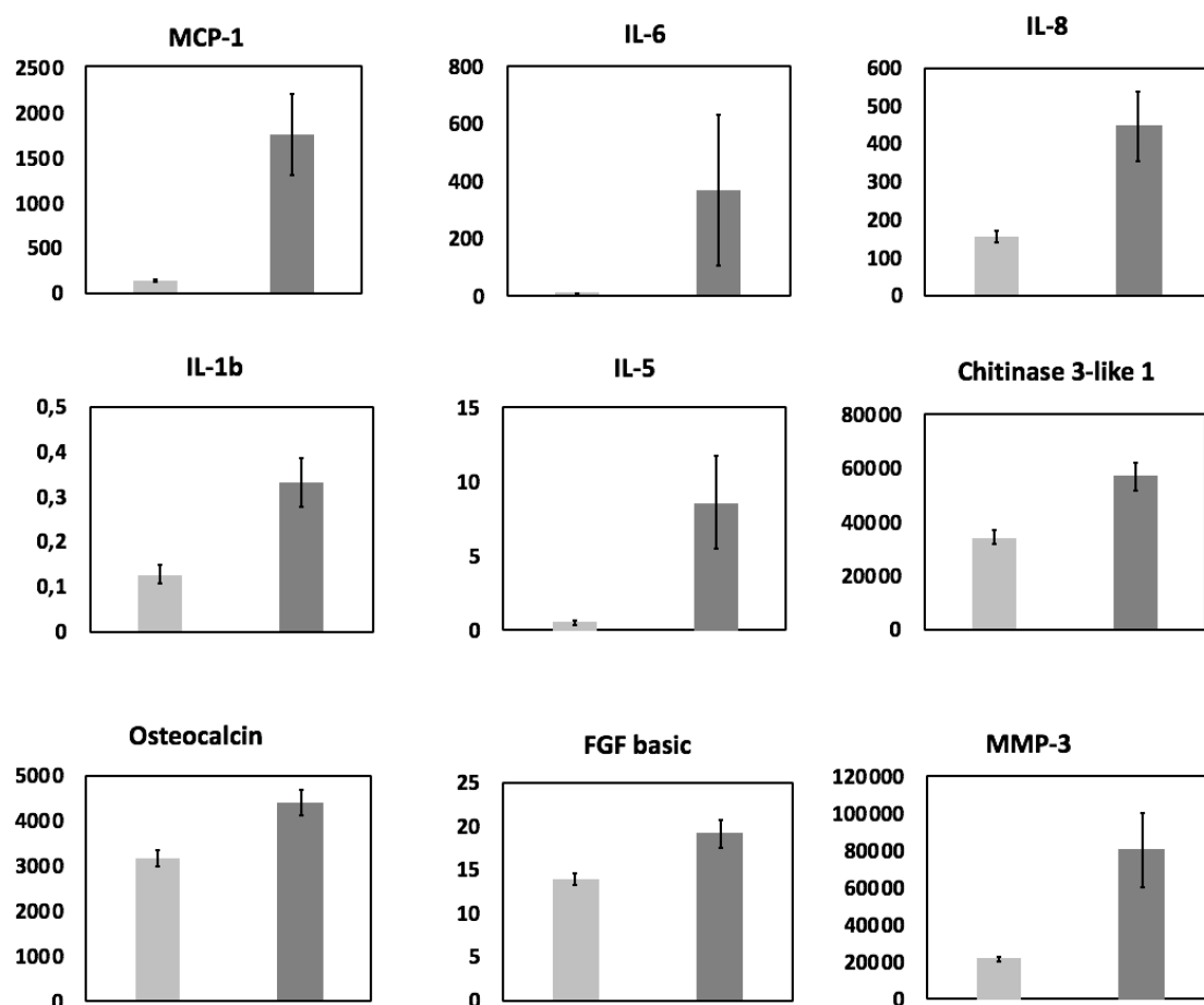
Figure 2. Bar plots representing the follicular fluid concentrations (pg/mL) of the nine cytokines found significantly different between endometriosis (dark gray) and control (light gray) patients. All patients ( n = 87 ) were included and data were log-transformed before Student test. Benjamini-Hochberg correction was applied to observed p -values for correction of risk I inflation. Error bars represent standard error of the mean (S.E.M.).
