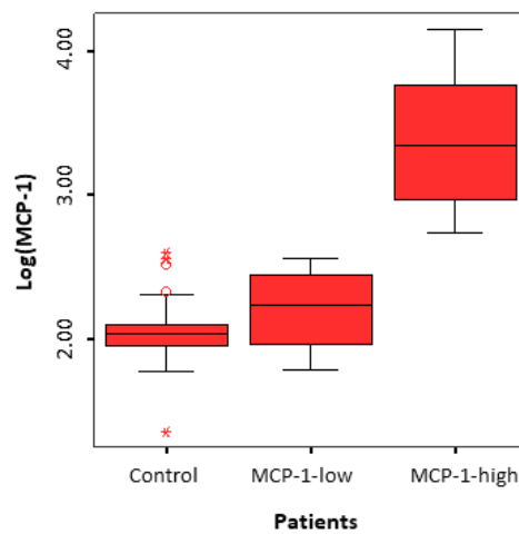
Figure 4. MCP-1 levels (following Log transformation) in the follicular fluid of patients with endometriosis (MCP-1-low and MCP-1-high subgroups) and controls.
