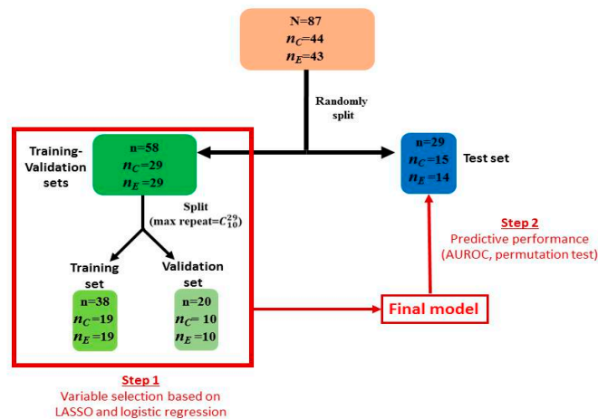
Figure 1. Multivariate analysis was conducted using training-validation (~ 2/3 of all data) and test sets (~1/3 of all data) strategy. Final model (containing variables selected in step 1) predictive capabilities were assessed in the test set to avoid validating overfitted models. Methods used in step 1 included LASSO, then logistic regression. Best models here were selected as those yielding AUROC > 0.95 in the validation set. Variables with no null estimated coefficients were included in a logistic regression model and submitted to a backward procedure. Finally, the best model obtained was applied to the test set to confirm its performance based on the AUROC. Coefficient in the logistic regression were estimated as median of the coefficient of the best models in step 1. Legend: n_C , n_E : number of patients in the control and endometriosis group, respectively; LASSO: Least Absolute Shrinkage and Selection Operator; LR: logistic regression.
