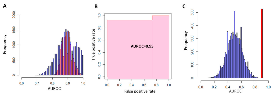
Figure 3. Performances of the LR models in the training-validation sets (A) and the test set (B,C). After LASSO, LR models with downregulation or stimulation protocol and MCP-1 as predictor variables were built and applied to the training and the validation sets. Histograms of AUROC show, as expected, good predictive performance of this models on the training set (red bars in (A)). Median AUROC in the validation sets was similar to the one found with the training set (~ 0.90) but exhibited more dispersion (blue bars in (A)). When the response vector in the test set was permuted, the performance of the model was indistinguishable from that of the random model (median and mean AUROC equal to 0.5, blue bars in (C)) and very different for the predictive capability of the model on the original response vector (AUROC = 0.95, red bar in (C)).
