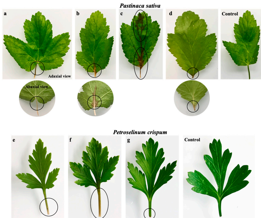
Figure 3. Leaf immersion assay. Phytotoxic damage of \alpha -acetylcholinol (1) and p -hydroxybenzoic acid (2) on leaves excised from parsnip ( P. sativa ) and parsley ( P. crispum ) plants: (a) p -hydroxybenzoic acid (7.25 mM), (b) p -hydroxybenzoic acid (14.5 mM), (c) p -hydroxybenzoic acid (22.0 mM), (d) \alpha -acetylcholinol (22.0 mM), (e) p -hydroxybenzoic acid (14.5 mM), (f) p -hydroxybenzoic acid (22.0 mM), and (g) \alpha -acetylcholinol (22.0 mM). The sterile uninoculated medium was used as a control. The circle indicates the phytotoxic effect.
