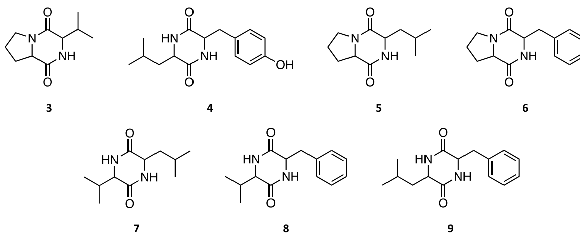
Figure 5. Minor diketopiperazines identified in the crude extract of A. dauci ; cyclo-(pro-val) (3), cyclo-(leu-tyr) (4), cyclo-(pro-leu) (5), cyclo-(pro-phe) (6), cyclo-(pro-phe) (6), cyclo-(val-leu) (7), cyclo-(val-phe) (8), and cyclo-(leu-phe) (9).
