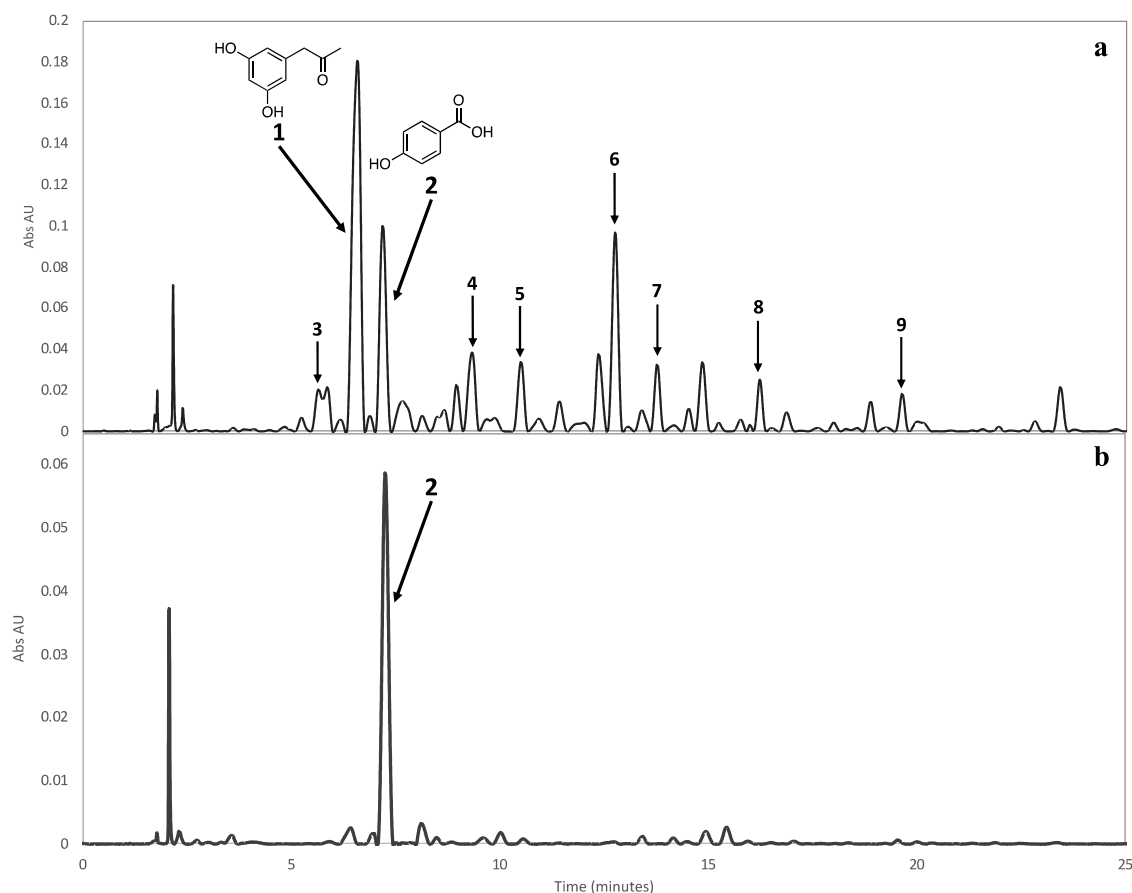
Figure 4. HPLC chromatographic profile of the medium polarity fraction from the extract of A. dauci at 96 h of culture. The chromatogram shows the peaks corresponding to \alpha -acetylrcinol (1), p -hydroxybenzoic acid (2), and the diketopiperazines (3–9) at (a) 210 and (b) 257 nm.
