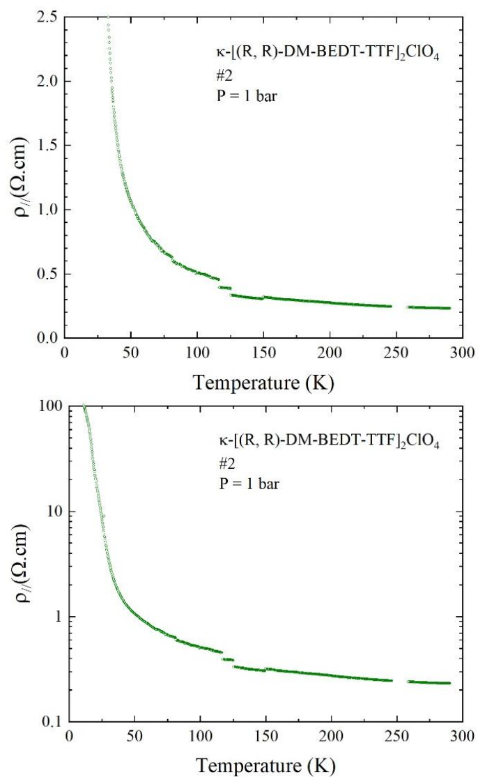
Figure S13. Temperature dependence of the in-plane electrical resistivity \rho_{\parallel}(T) for a single crystal of \kappa -[(R,R)-DM-BEDT-TTF] 2 ClO 4 (#2) at P = 1 bar in linear (top) and logarithmic (bottom) vertical scale.
