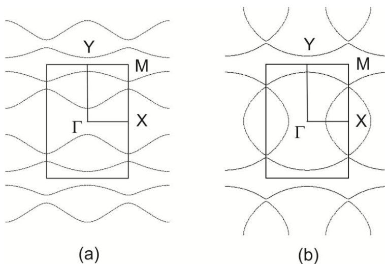
Figure S9. Extended Hückel Fermi surface for the two donor layers of \kappa -[(S,S)-DM-BEDT-TTF] 2 ClO 4 where the DFT hole transfer between the two layers is taken into account: (a) layer type 1, and (b) layer type 2.
