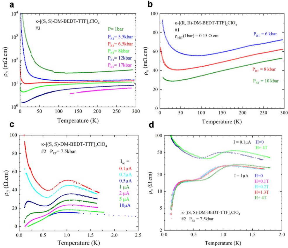
Figure 3. Temperature dependence of the in-plane electrical resistivity \rho_{//} for a single crystal of \kappa -[(S,S)-DM-BEDT-TTF] 2 ClO 4 (a) and for a single crystal of \kappa -[(R,R)-DM-BEDT-TTF] 2 ClO 4 (b) at different pressures. c) Temperature dependence of the electrical resistivity \rho_{//} for a single crystal (#2) of \kappa -[(S,S)-DM-BEDT-TTF] 2 ClO 4 in 4 points for different current intensities and under an applied pressure of 7.5 kbar. It shows a current induced insulator to metal transition below 1 K. d) Temperature dependence below 2 K of the in-plane electrical resistivity for a single crystal of \kappa -[(S,S)-DM-BEDT-TTF] 2 ClO 4 (#2) at 7.5 kbar plotted for two different applied currents and different magnetic fields applied perpendicularly to the (a,b) plane.
