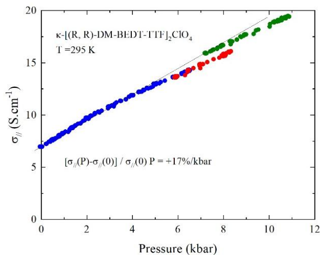
Figure S15. Pressure dependence of the in-plane electrical conductivity at room temperature for a single crystal of \kappa -[(R,R)-DM-BEDT-TTF] _2 ClO _4 (#1). The black line is the linear fit to the data.
