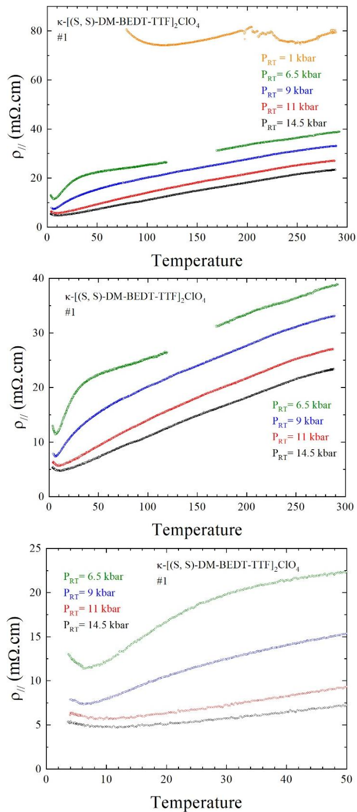
Figure S10. Temperature dependence of the in-plane electrical resistivity \rho_{||}(T) for a single crystal of \kappa -[(S,S)-DM-BEDT-TTF] 2 ClO 4 (#1) at different pressures, in the whole measured temperature range (two upper graphs) and below 50 K (bottom).
