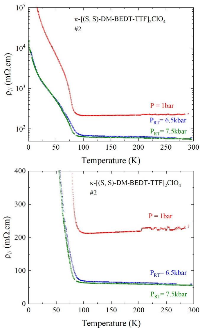
Figure S11. Temperature dependence of the in-plane electrical resistivity \rho_{//}(T) for a single crystal of \kappa\text{-}[(S,S)\text{-DM-BEDT-TTF}]_2\text{ClO}_4 (#2) at different pressures.
