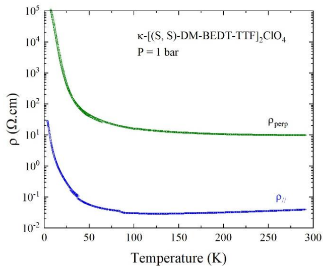
Figure S16. Temperature dependence of the in-plane \rho_{\parallel} and out-of-plane \rho_{\text{perp}} electrical resistivity for single crystals of \kappa -[(S,S)-DM-BEDT-TTF] _2 ClO _4 at ambient pressure.
