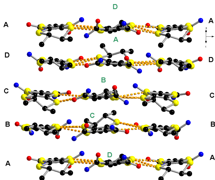
Figure 2. Packing in parallel stacks of the four types of molecules through short lateral S...S interactions along the b axis in [( S,S )- 1b ] 2 ClO 4 .
