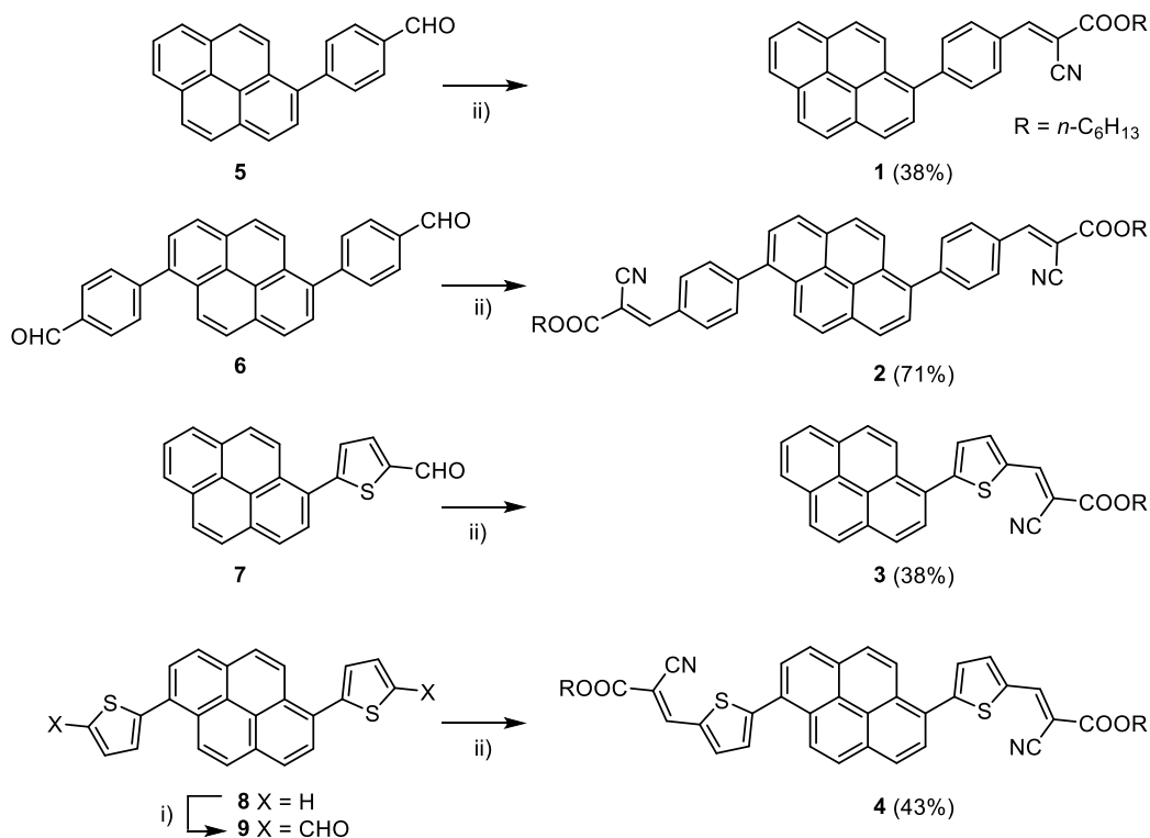
Scheme 1. Synthesis of the target compounds 1-4 . i) \text{POCl}_3 , DMF, dichloroethane ii) n -hexyl-cyanoacetate, \text{Et}_3\text{N} , \text{CHCl}_3 , reflux.
