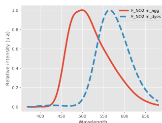
(1b) Emission spectra of the Fluoro-Nitro combination for the "mix of aggregates" and the "mix of dyes" cases
