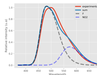
(1c) Graph showing that the emission spectra of the Fluoro-Nitro mix of aggregates can be seen as the weighted sum of the emission spectra of Fluoro and Nitro pure compounds.
