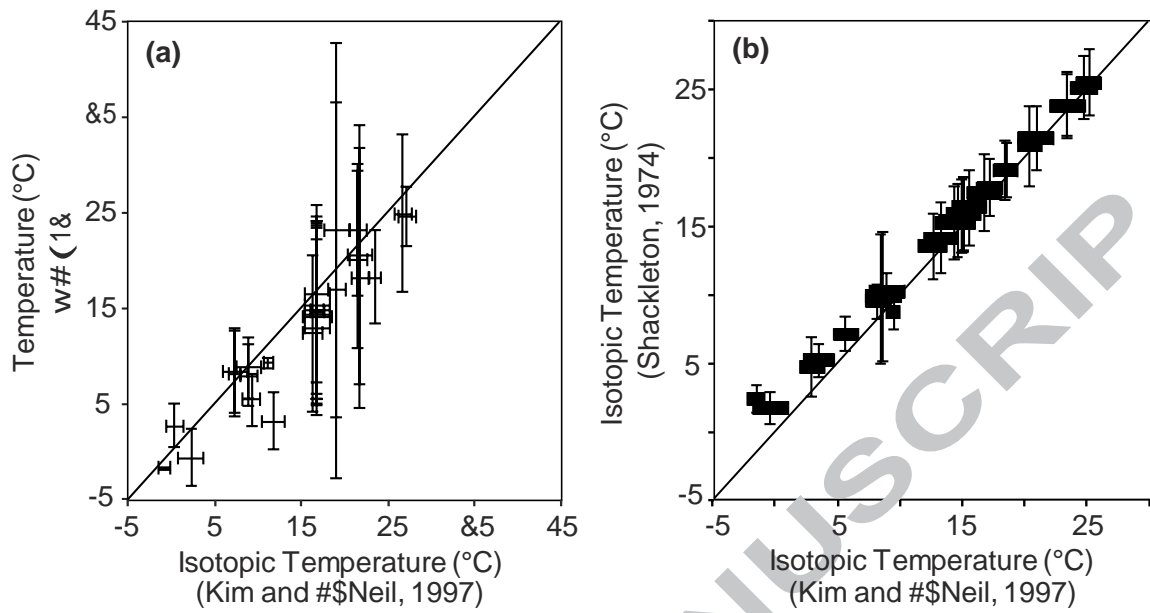
Figure 5: Independent temperature comparison from (a) WOA13 and oxygen isotopic data using the Kim and O'Neil (1997) equation and (b) oxygen isotopic temperatures computed with Shackleton (1974) and Kim and O'Neil (1997) equations.
