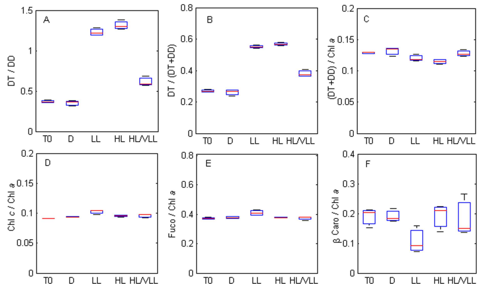
Fig 4. Comparison between pigment ratios ( g\ g^{-1} , experiment 1) measured before (T0) and after exposure to different light levels (D, LL, HL, HL/VLL). A. Ratio diatoxanthin / diadinoxanthin. B. Ratio diatoxanthin / xanthophyll cycle pigments (diadinoxanthin + diatoxanthin). C. Ratio xanthophyll cycle pigments / chlorophyll a. D. Ratio chlorophyll c / chlorophyll a. E. Ratio fucoxanthin / chlorophyll a. F. Ratio \beta -carotene / chlorophyll a.
