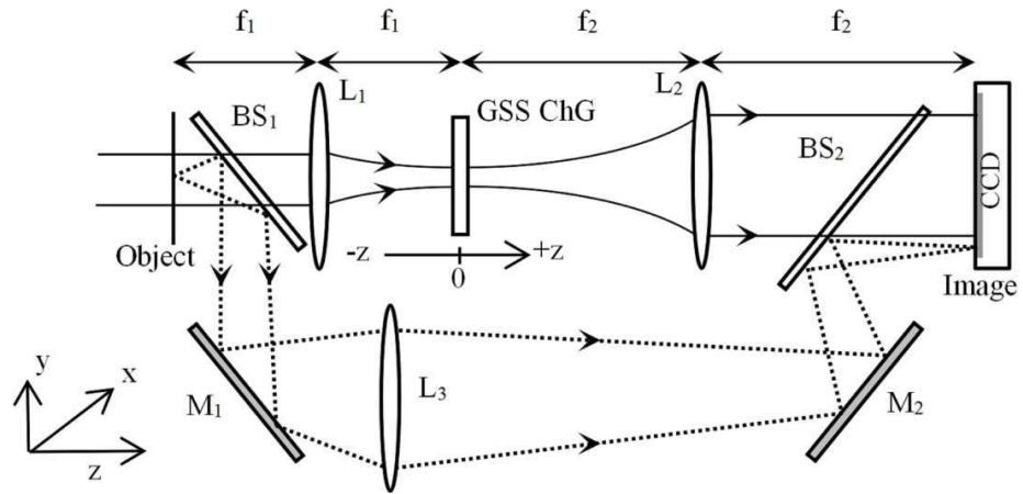
Fig. 1. Experimental D4 \sigma -Z-scan setup. The GSS ChG sample is scanned along the beam direction around the focal plane ( z=0 ). The labels refer to: lenses (L 1 , L 2 and L 3 ), beam splitters (BS 1 and BS 2 ), mirrors (M 1 and M 2 ), Camera (CCD).
