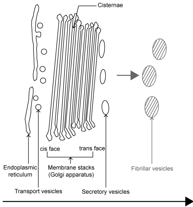
Fig. 8. Schematic ultrastructure and relations between the reticulum endoplasmic, Golgi apparatus and fibrillar vesicles in the foraminiferal cell.
