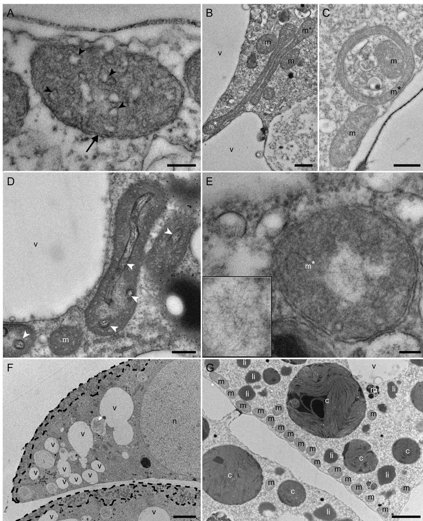
Fig. 5. Transmission electron micrographs of benthic foraminiferal mitochondria.
