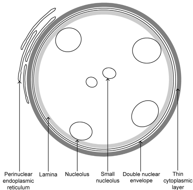
Fig. 4. Schematic ultrastructure of a foraminiferal nucleus.
