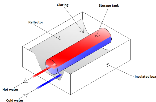
Fig. 4. Integrated collector storage system.
