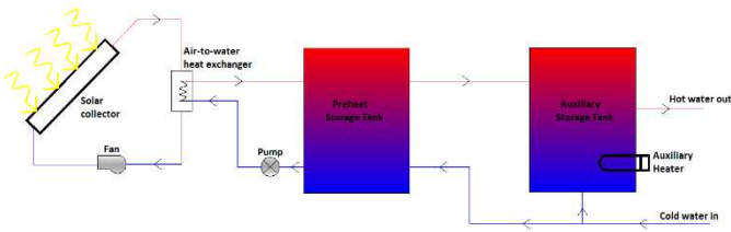
Fig. 6. Air system.
