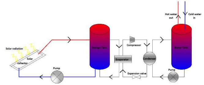
Fig. 6. Indirect series solar heat pump.
