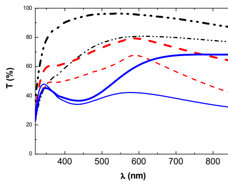
Figure 15: Colour change induced by polarization inversion in different EC-devices : (- - - - -) ITO//ITO, (- - - - -) \text{WO}_3 / \text{Ag} / \text{Cu} : \text{Al} / \text{WO}_3 // \text{ITO} and (—) \text{WO}_3 / \text{Ag} / \text{Cu} : \text{Al} / \text{Pt} / \text{WO}_3 // \text{ITO} .
