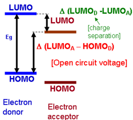
Fig. 1. Band structure of the interface donor/acceptor.
