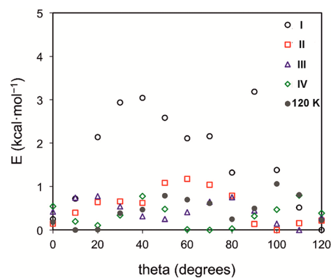
Figure 5. Computed energy profiles (in kcal mol -1 ) for the rotation of each independent rotator surrounded by their neighbor molecules; the five models for the DFT transition structures are described in Figure S11.
