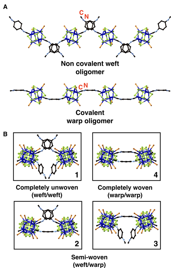
Figure 3. (A) The protocloth consists of unwoven, oligomeric weft segments and woven oligomeric warp segments. (B) Different possible configurations of crossing points in the warp (woven) and weft (unwoven) strands. The warp and weft strands that make up the protocloth are polydisperse in length. The warp/warp combination does not occur in the crystal.
