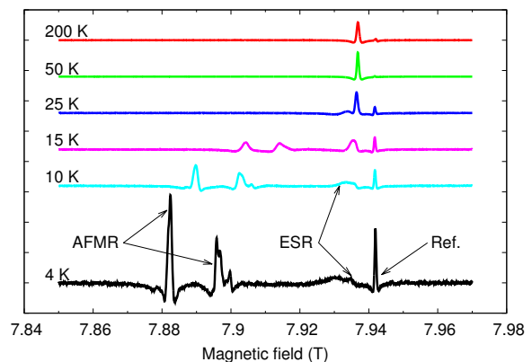
FIG. 2: Temperature dependence of the ESR and AFMR spectra in an EDT 2 AsF 6 crystal with B_0 \parallel \mathbf{a} , 222.4 GHz. The AFMR below 25 K signals an antiferromagnetic order in large regions. The ESR from paramagnetic regions persists to low temperatures. Reference at 7.941 T is KC 60 .
