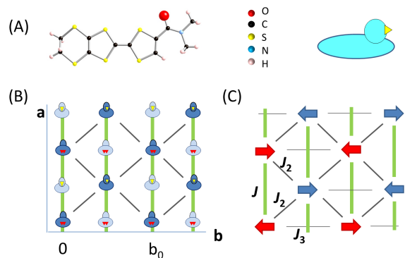
FIG. 1: (A) The EDT molecule and its schematic representation as a duck in further panels. (B) Schematic structure of the (\mathbf{a}, \mathbf{b}) plane of EDT 2 AsF 6 . Dark and light ducks represent charge rich and charge poor molecules. (C) The frustrated, isosceles triangular magnetic lattice. J , J_2 and J_3 are the first, second and third neighbor isotropic antiferromagnetic exchange interactions respectively. The exchange is large along chains while frustration cancels the isotropic interactions between chains.
