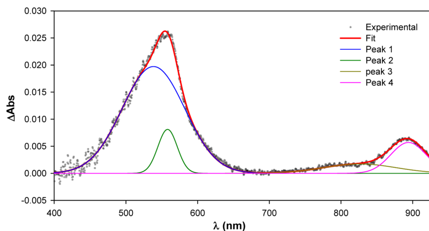
Figure 6. Variation of the UV–visible spectrum of 4a in acetonitrile (0.21 mM) with (\text{TBA})\text{PF}_6 (0.1 M) as electrolyte on a platinum electrode at 0.59 V.
