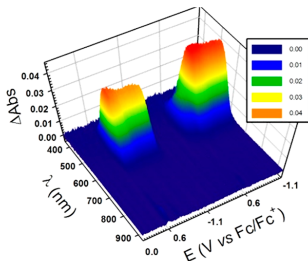
Figure 5. Spectroelectrochemistry in TLCV conditions ( \sim 50 \mu\text{m} ; 100 \text{ mV}\cdot\text{s}^{-1} ) of BtBoX (0.2 mM) in acetonitrile with (\text{TBA})\text{PF}_6 (0.1 M) as electrolyte on a platinum electrode.
