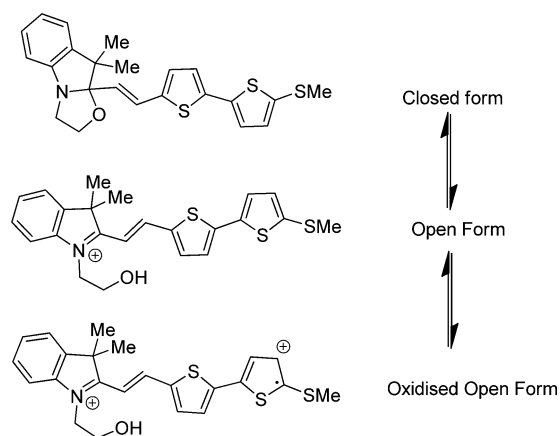
Scheme 4. Proposed Structure of the Three Metastable States of the Dyad Indolinoxazolidine–Bithiophene
