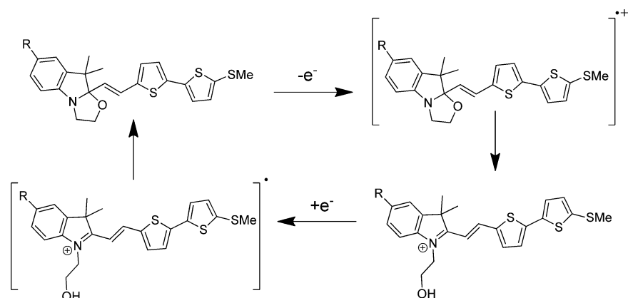
Scheme 4. Proposed Structure of the Three Metastable States of the Dyad Indolinoxazolidine–Bithiophene
