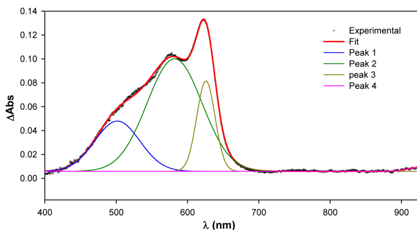
Figure 9. Variation of the visible spectrum of 4a in acetonitrile (0.21 mM) with (\text{TBA})\text{PF}_6 (0.1 M) as electrolyte on a platinum electrode at 0.81 \text{ V} .
