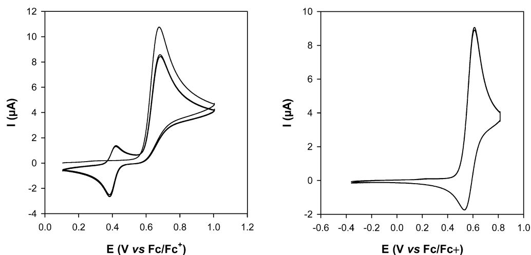
Figure 4. CV of 1a (left) and 1b (right) in acetonitrile (1 mM) with (TBA)PF 6 (0.1 M) on Pt working electrode at 100 mV·s -1 .
