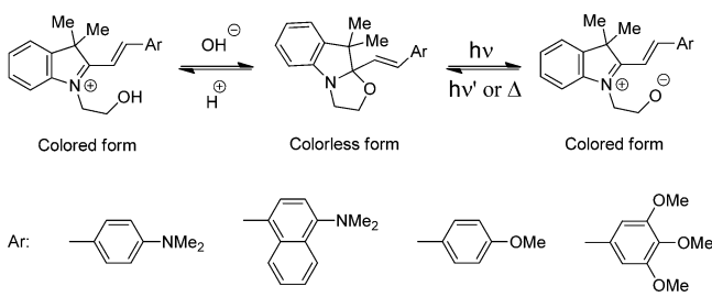
Scheme 1. Photo- and Acidochromic Equilibrium of Several Indolinooxazolidine Analogues Used as Multiaddressable Switches in Nonlinear Optics 30
