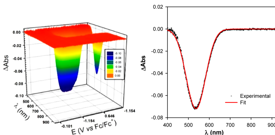
Figure 7. (left) Spectroelectrochemistry in TLCV conditions ( \sim 50 \mu\text{m} ; 100 \text{ mV}\cdot\text{s}^{-1} ) of irradiated BtBoX (0.2 mM) in acetonitrile with (\text{TBA})\text{PF}_6 (0.1 M) as electrolyte on a platinum electrode. (right) Variation of UV–visible spectrum of an irradiated solution of 4a in acetonitrile (0.21 mM) with (\text{TBA})\text{PF}_6 (0.1 M) as electrolyte on a platinum electrode at -1.15 \text{ V} .
