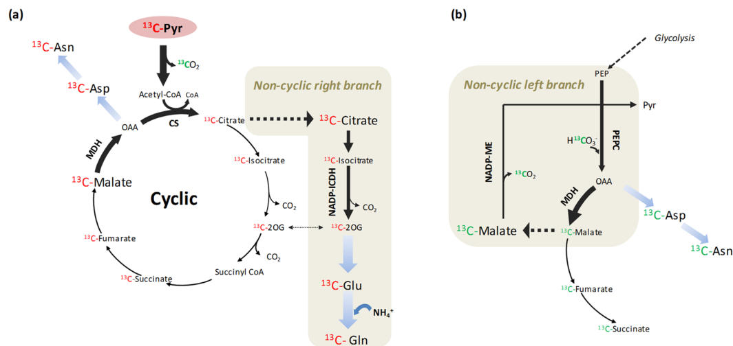
Figure 7. TCA cycle flux modes inferred from the ^{13}\text{C} -Pyr-labelling of wheat roots preadapted to ammonium nutrition. (a) Cyclic respiratory cycle and non-cyclic right branch for 2-OG (2-oxoglutarate) provision. The principal amino acid formation is also indicated. (b) Non-cyclic left branch with the participation of anaplerotic enzymes. The re-assimilation of ^{13}\text{C} label coming from ^{13}\text{C} -Pyr decarboxylation step is indicated in green. TCA cycle-related enzyme activities that were determined in wheat roots are indicated (CS, MDH, NADP-ICDH, NADP-ME, and PEPC).
