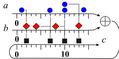
Figure 2: Synchronization of two sequences \{a\} \oplus \{b\}
