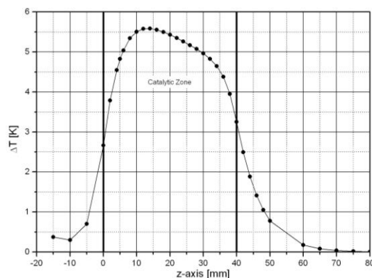
Fig. 9. The \Delta -temperature between the catalyst bed and the furnace wall, H_2O/CH_3OH ratio of 1.36; CH_3OH molar feed rate is 1.16 \cdot 10^{-4} \text{ mol.s}^{-1}
