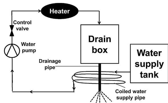
Fig. 2. Schematic of the constructed prototype.
