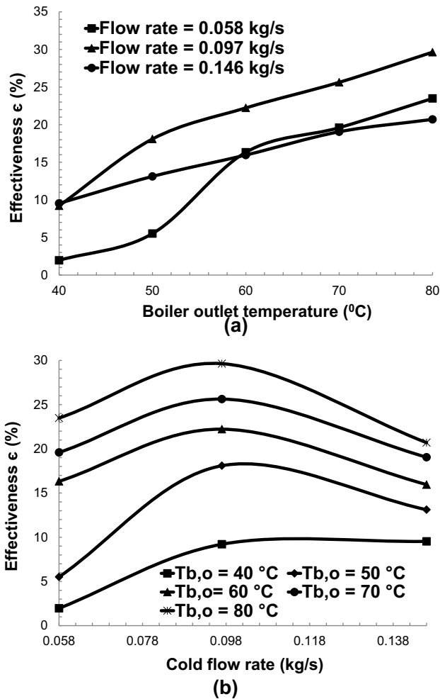
Fig. 10. Variation of the exchanger effectiveness (a) in function of the boiler outlet temperature for different cold flow rates and (b) in function of the cold flow rate for different boiler outlet temperatures.
