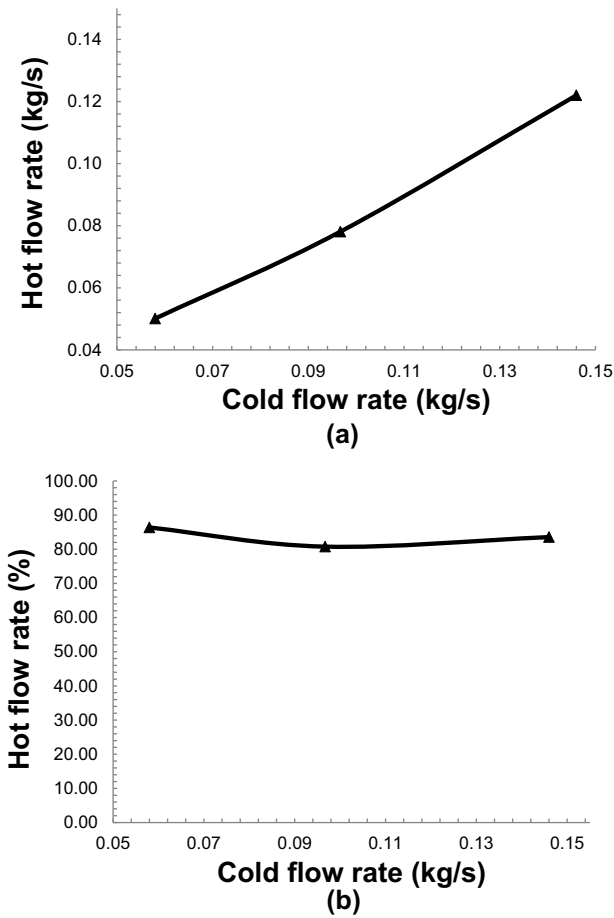
Fig. 5. Variation of (a) hot water flow rate and (b) percentage of hot water flow rate in terms of the cold water flow rate.
