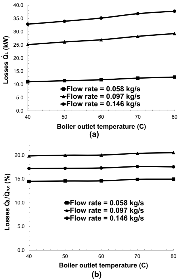
Fig. 8. Variation of (a) losses and (b) percentage of losses in function of the boiler outlet temperature for different cold flow rates.
