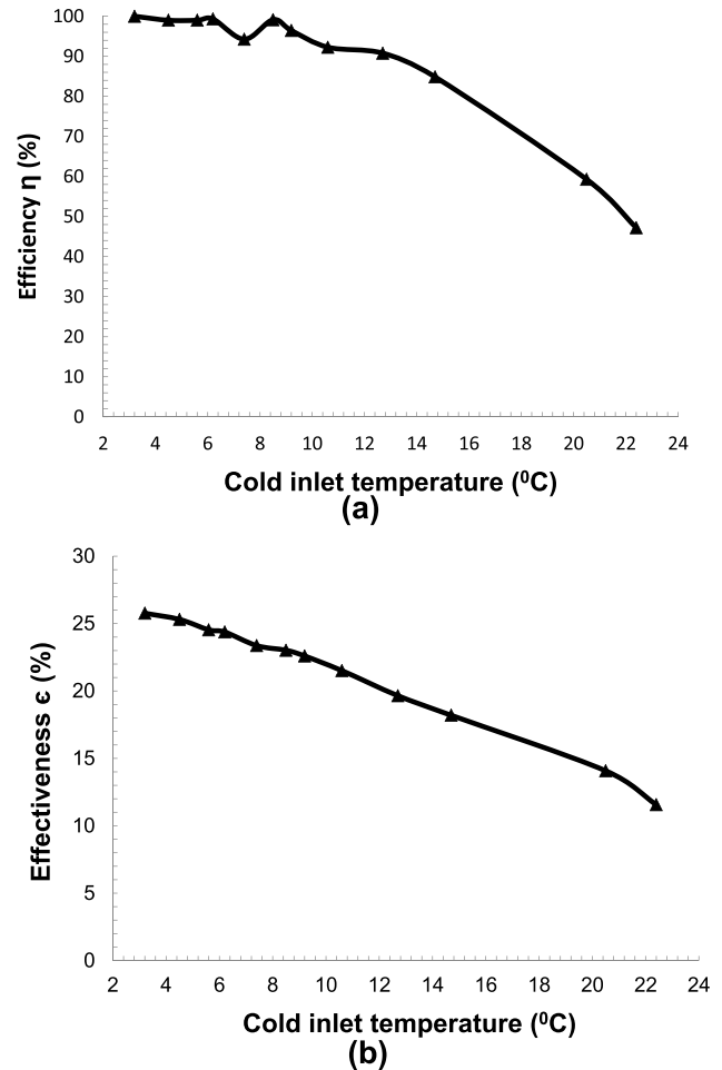
Fig. 7. Variation of (a) efficiency and (b) effectiveness of the recovery system in function of the cold inlet temperature.
