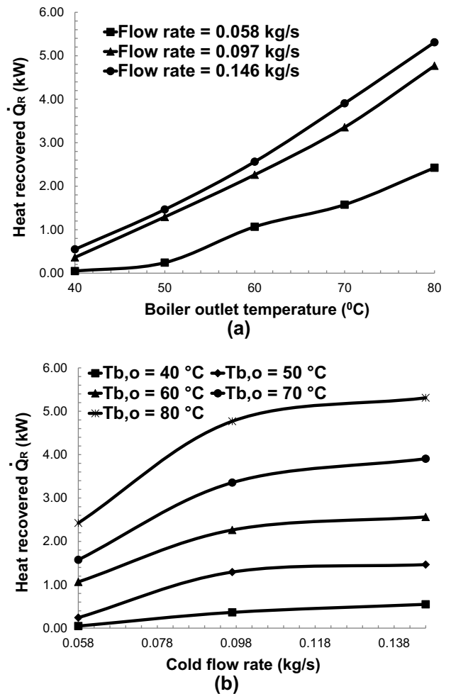
Fig. 9. Variation of recovered heat (a) in function of the boiler outlet temperature for different cold flow rates and (b) in function of the cold flow rate for different boiler outlet temperatures.
