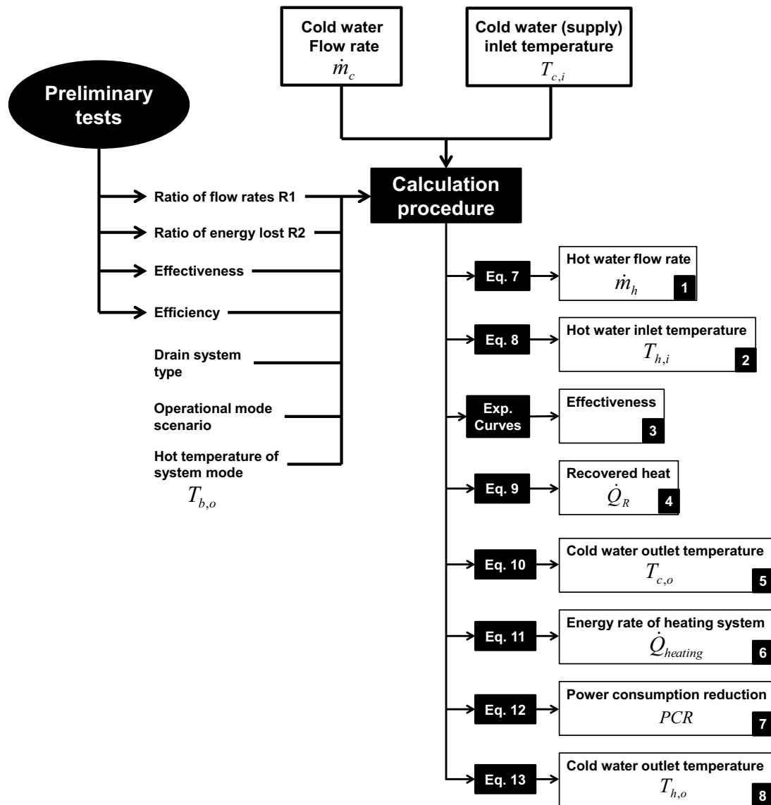
Fig. 11. Flow chart of the calculation procedure.
