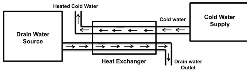
Fig. 1. Drain water heat recovery system (DWHR) working principle.
