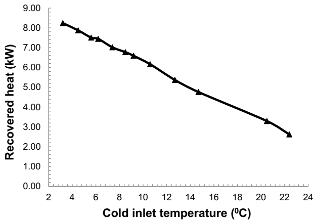
Fig. 6. Heat recovered in function of the cold inlet temperature.
