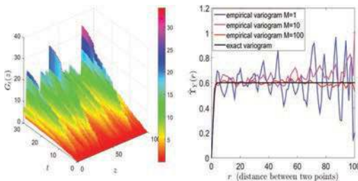
Figure 1. Left: example of one realization of G_t(\cdot) , right: variogram ( l_c = 1, \nu = 2, \sigma^2 = 0.6 ).
