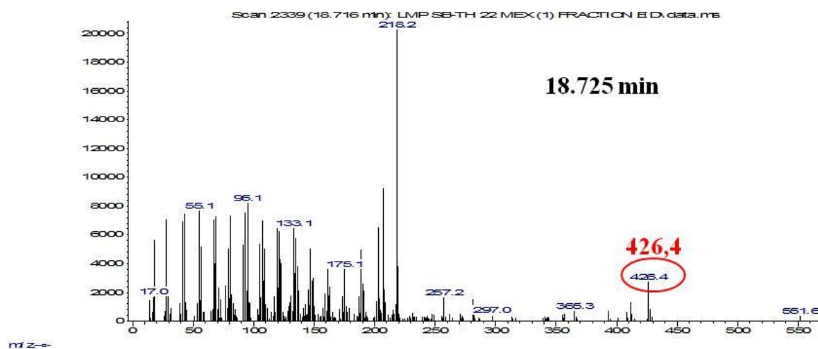
Fig. S3b. MS spectra of components in fraction B
