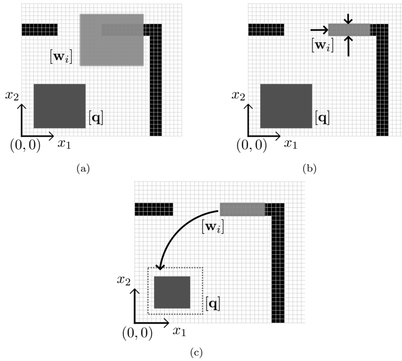
Figure 6. Example of contraction. In Figure 6(a) there is a grid map G (each black cell value is 1). The box [w_i] (light grey) is a guaranteed evaluation of the measurement w_i according to [q] (dark grey) and [y_i] . By using the constraint a measurement has to intersect an obstacle in the map the domain [w_i] is contracted (Figure 6(b)) and then by using another constraint ( the distance between the robot and the detected obstacle is y_i \in [y_i] ) it is possible to contract the domain [q] (Figure 6(c)).
