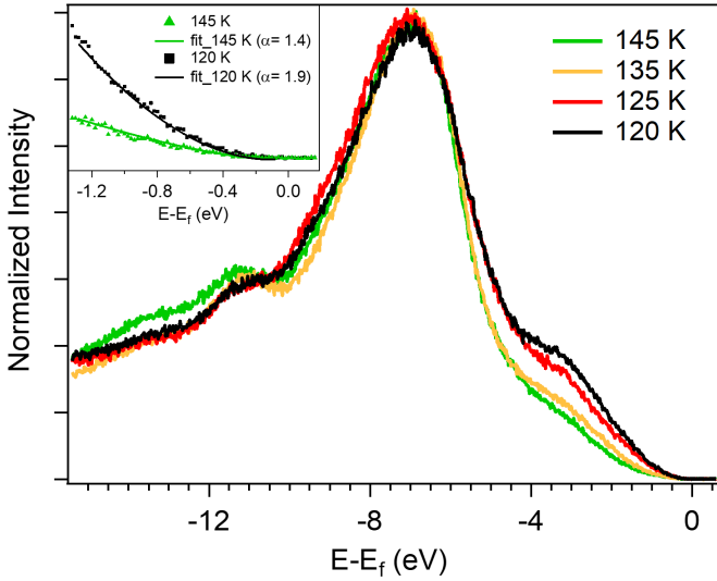
Fig. 2. Photoemission spectra of the \alpha -(BEDT-TTF) _2 I _3 for different temperatures, above and below the metal-insulator transition temperature. All spectra are renormalized with respect to the peak at -7 eV. No Fermi edge is observed in the whole experimental range of temperatures, especially in the metallic phase of the \alpha -(BEDT-TTF) _2 I _3 at T > 135 K. Inset: In the vicinity of the Fermi level, the spectral weight behaves as a power law with an exponent \alpha > 1 , signature of a strongly correlated Luttinger liquid (a convolution with experimental resolution of 15 meV has been taken into account).
