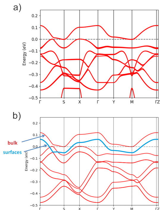
Fig. 5. DFT calculated band structure for the \alpha -(BEDT-TTF) _2 I _3 model at room temperature using c' = 5c . a) : Stoichiometric surface; the band structure of the bulk (Figure 3a) is found to be practically identical. Note that, for the case of the surface, the bottom of the band structure looks a bit different because of the emergence of some I _3^- bands in that region. b) : Modelling the effect of a defect of I _3^- units (see text).
