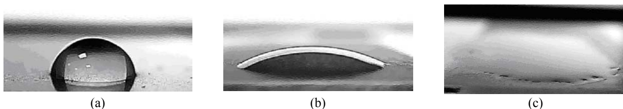
Fig. 9 – Image of water contact angle on the surface of: a) non annealed \text{TiO}_2 film; b) annealed \text{TiO}_2 film; c) annealed \text{TiO}_2 film after strong UV light exposure for 30 min.
