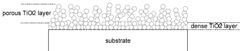
Fig. 7 – Schematic representation of \text{TiO}_2 layer deposited by spray pyrolysis method.
