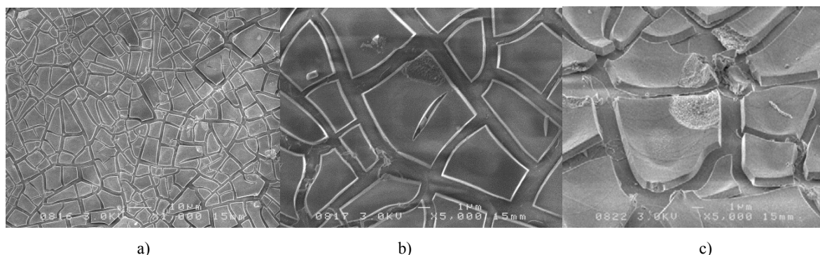
Fig. 8 – SEM images of ‘channeled’ \text{TiO}_2 layer: a) \times 1000 ; b) \times 5000 ; c) \times 5000 tilted image.
