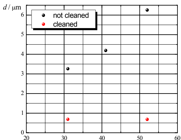
Fig. 6 – \text{TiO}_2 layer thickness d vs. times of spray phase before and after porous layer removing. Thin films preparation: substrate temperature 270 °C, spray phase 1 s, pause ~10 s, pressure 1.3 bar, nozzle size 0.5 mm, samples were annealed at 300 °C for 20 min and 500 °C for 20 min.
