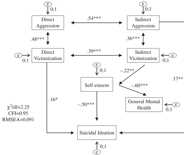
Figure 2. Analysis of relationships between forms of peer aggression, self-esteem, general health and suicidal ideation for boys ( n = 151 ). Note: *p < 0.05 ; **p < 0.01 ; ***p < 0.001 . \chi^2/df , degree of freedom; CFI, comparative fit index; RMSEA, root mean square error of approximation
