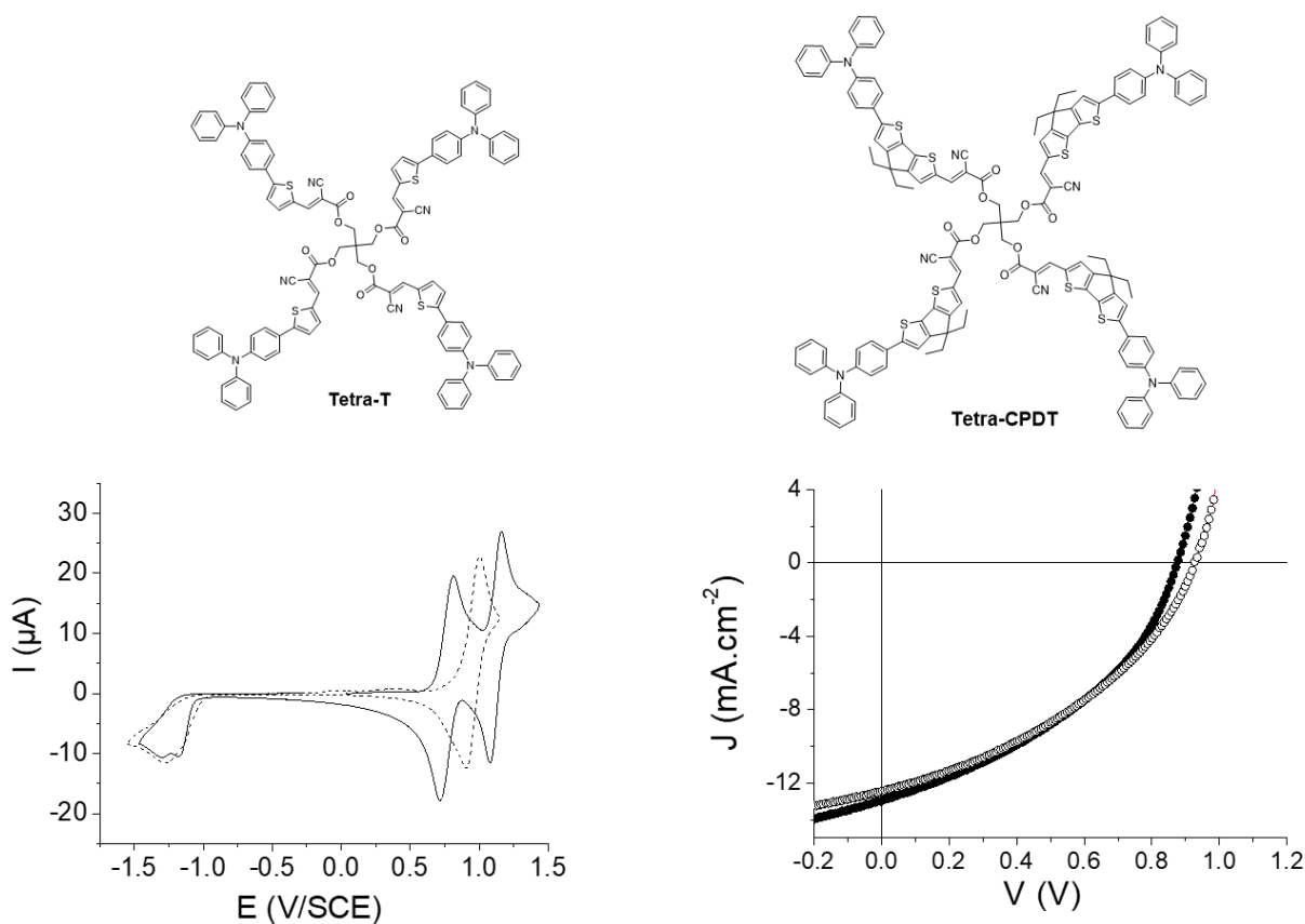
Figure 12: CV of Tetra-T (dashed line) and Tetra-CPDT (solid line) 0.5 \text{ mM} in 0.1 \text{ M Bu}_4\text{NPF}_6/\text{CH}_2\text{Cl}_2 , Pt working electrode, scan rate 100 \text{ mV}/\text{s} and current density vs voltage curves of BHJ OSCs prepared from Tetra-T (white circles) and Tetra-CPDT (black circles) under AM 1.5 white light illumination at 100 \text{ mW}/\text{cm}^2 . Adapted from reference 116 by permission of The Royal Society of Chemistry .
