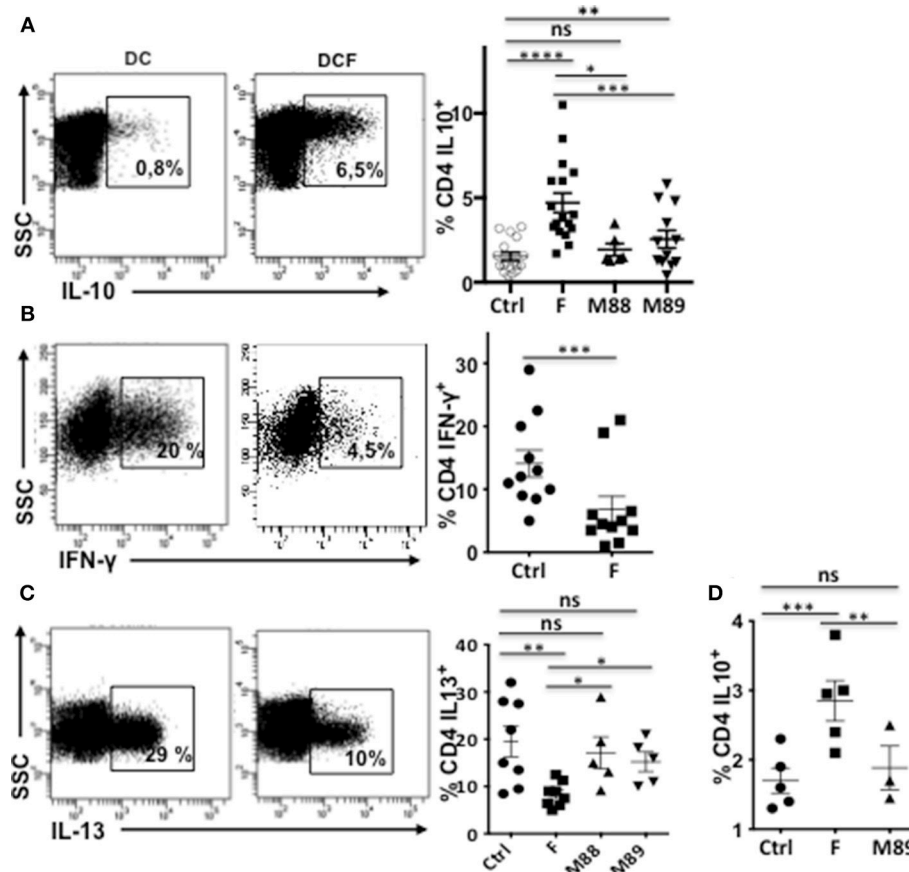
FIGURE 1 | Exposure to F. prausnitzii (F) promotes DC ability to prime IL-10-secreting T cells. VPD-stained naïve CD4 ^{+} T cells were stimulated by LPS-stimulated DC, pre-exposed or not to indicated bacteria at day 0 [(A) n = 6-18 , (B) n = 11 , (C) n = 5-7 ] or from day 4 to 6 of their differentiation [(D) n = 5 ], and were re-stimulated by CD3/CD28 beads. Representative examples and mean percentages \pm sem of CD4 ^{+} T cells expressing indicated cytokines. Paired t -test: * p < 0.05 , ** p < 0.005 , *** p < 0.0005 , and **** p < 0.00005 .
