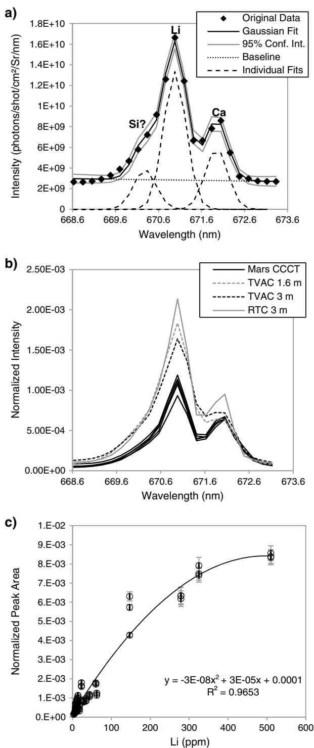
Figure 1. (a) Example Gaussian fit for the Li 671 nm peak on the RTC spectrum for Norite. (b) Comparison of Norite spectra taken on Mars (CCCT), TVAC 1.6 m and 3 m, and the RTC. (c) Univariate peak area model for Li.
